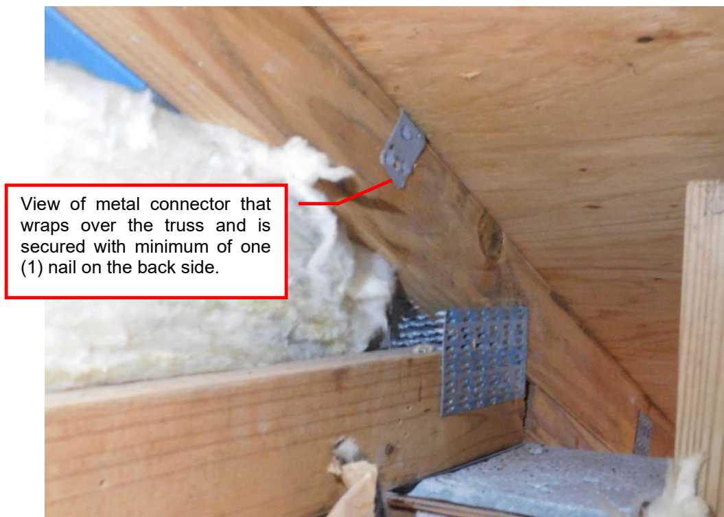
View of metal connector used on Roof to Wall attachment (per question 4).
